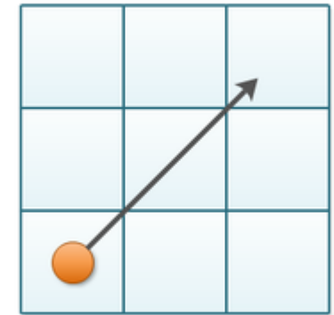
Euclidean Distance
